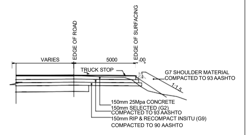
TRUCK STOP CROSS SECTION SCALE 1:300
