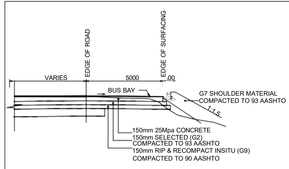
BUS BAY CROSS SECTION N.T.S
