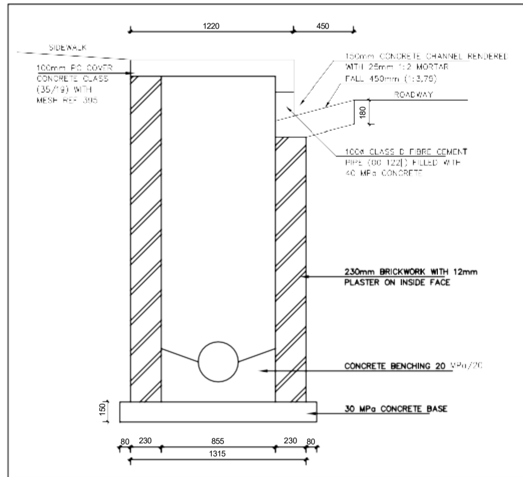
SECTION THROUGH KERB INLET SHAFT TO PIPE N.T.S
