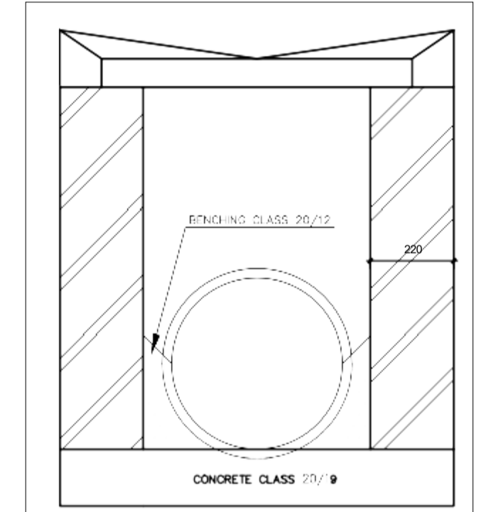
SECTION THROUGH KERB INLET SHAFT TO PIPE N.T.S
