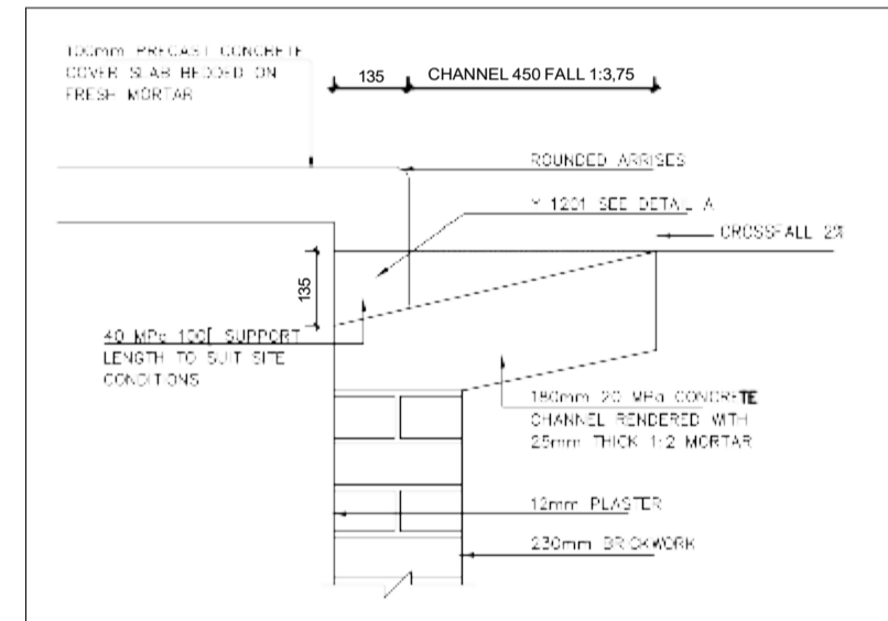
DETAIL OF CHANNEL & KERB INLET OPENING N.T.S
