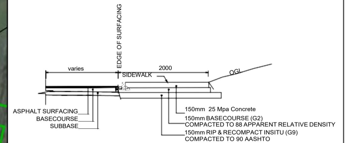
TRUCK STOP CROSS SECTION SCALE 1:300
