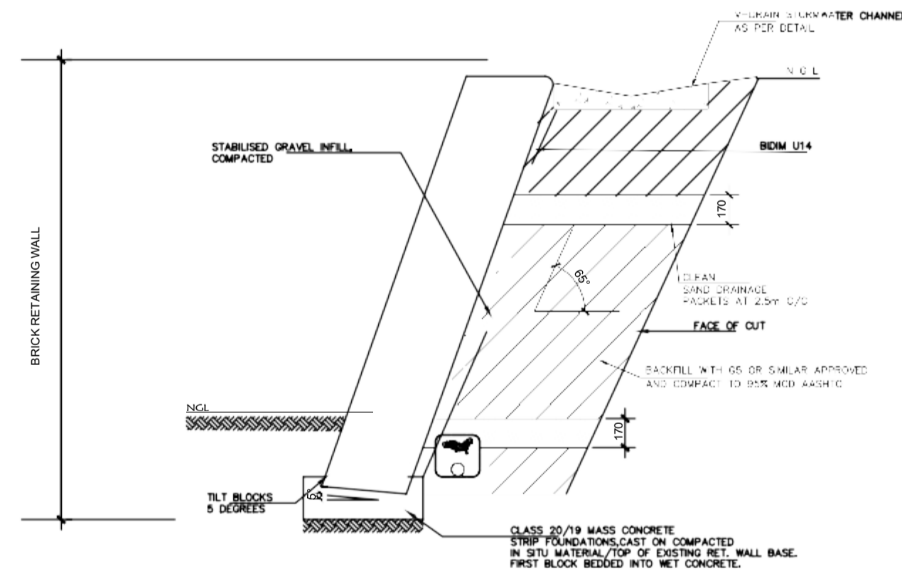
RETAINING WALL SECTION N.T.S
