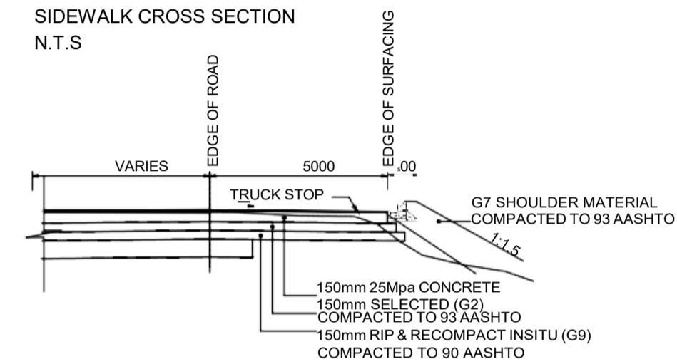
TRUCK STOP CROSS SECTION N.T.S
