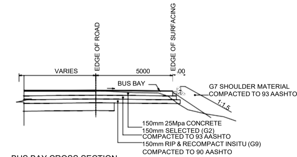
BUS BAY CROSS SECTION N.T.S
