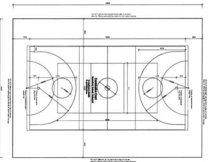
COMBINATION COURT DETAILS SCALE 1:50
